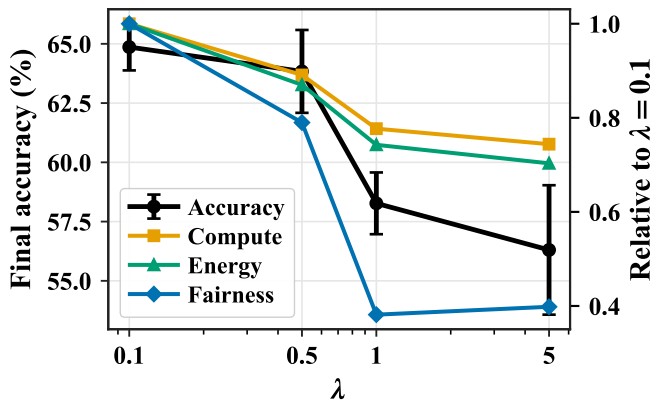
CIFAR-10
